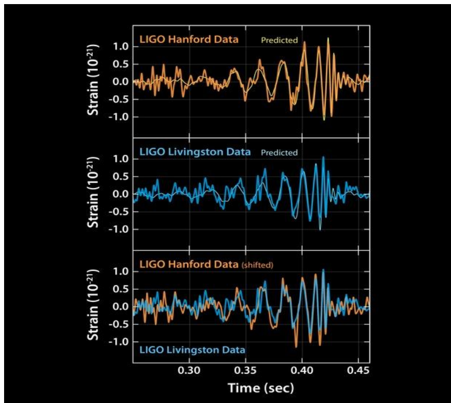
Gravitational waves as predicted by Einstein ( LIGO ) [4]
