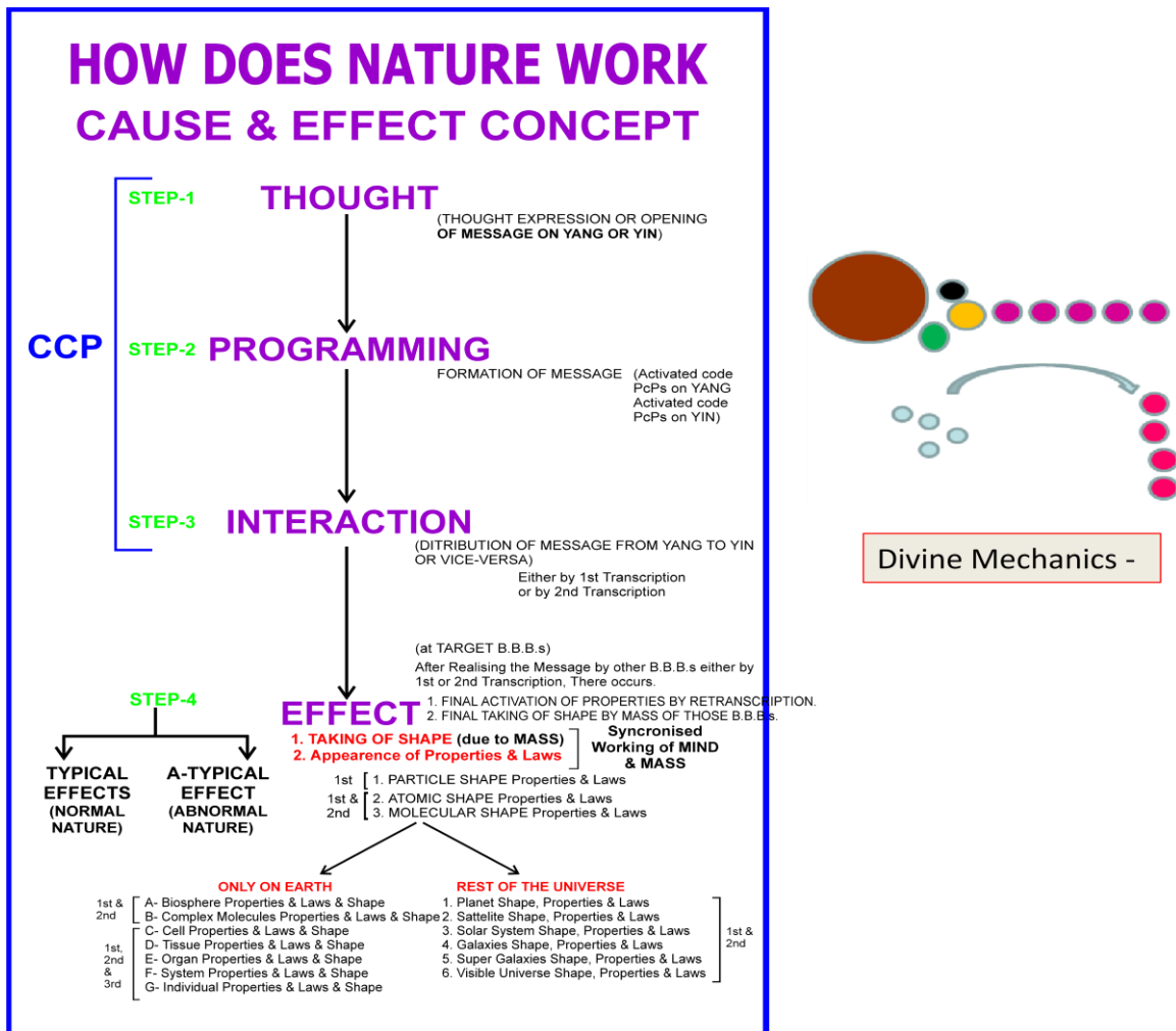
Fig. 6 Divine Mechanics – How Does Nature work ?
