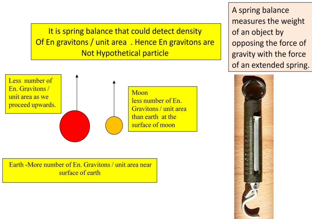
Fig 13.2 A spring balance measures the weight of an object by opposing the force of gravity with the force of an extended spring. Thus detecting density of EGs /unit area confirming their existence.
