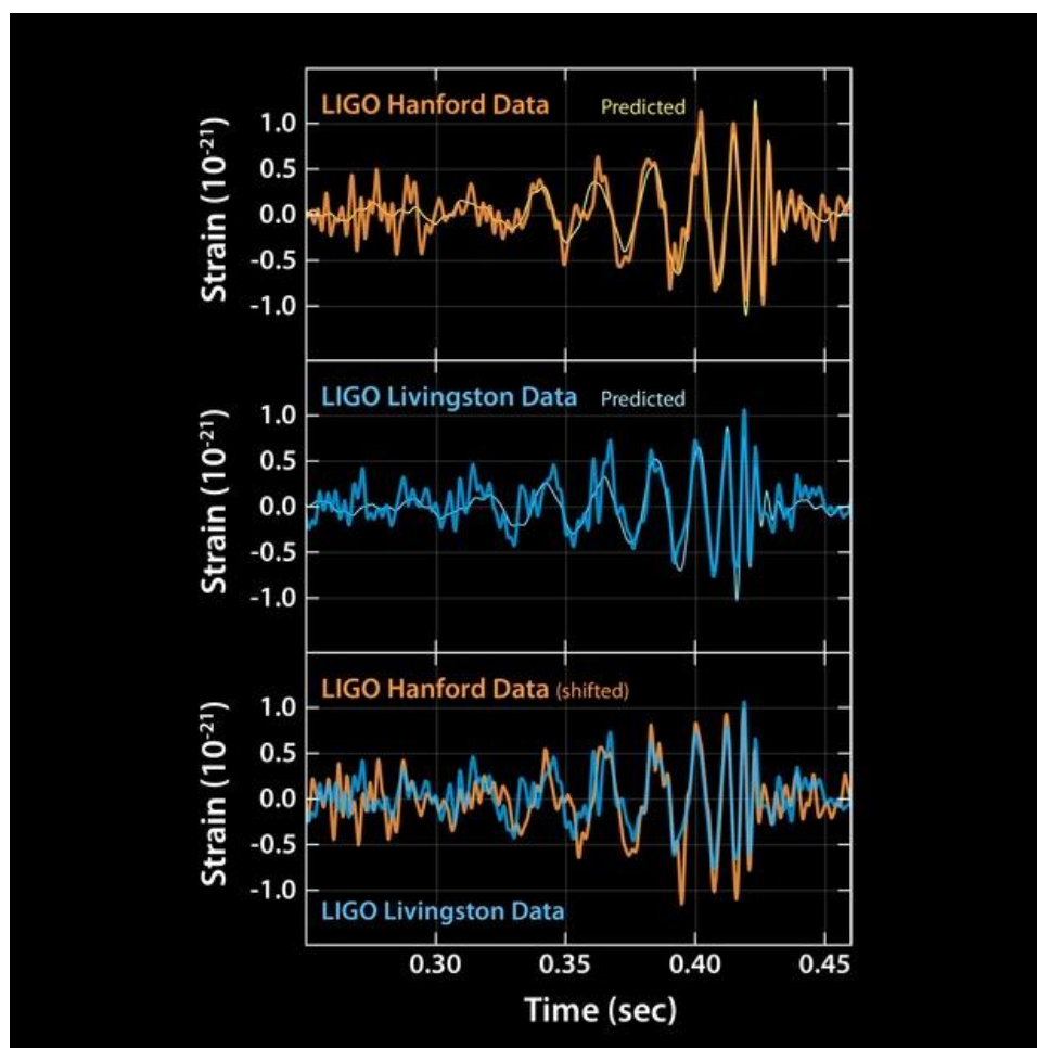
Fig 21 – So called gravitational waves as predicted by Einstein ( LIGO )
