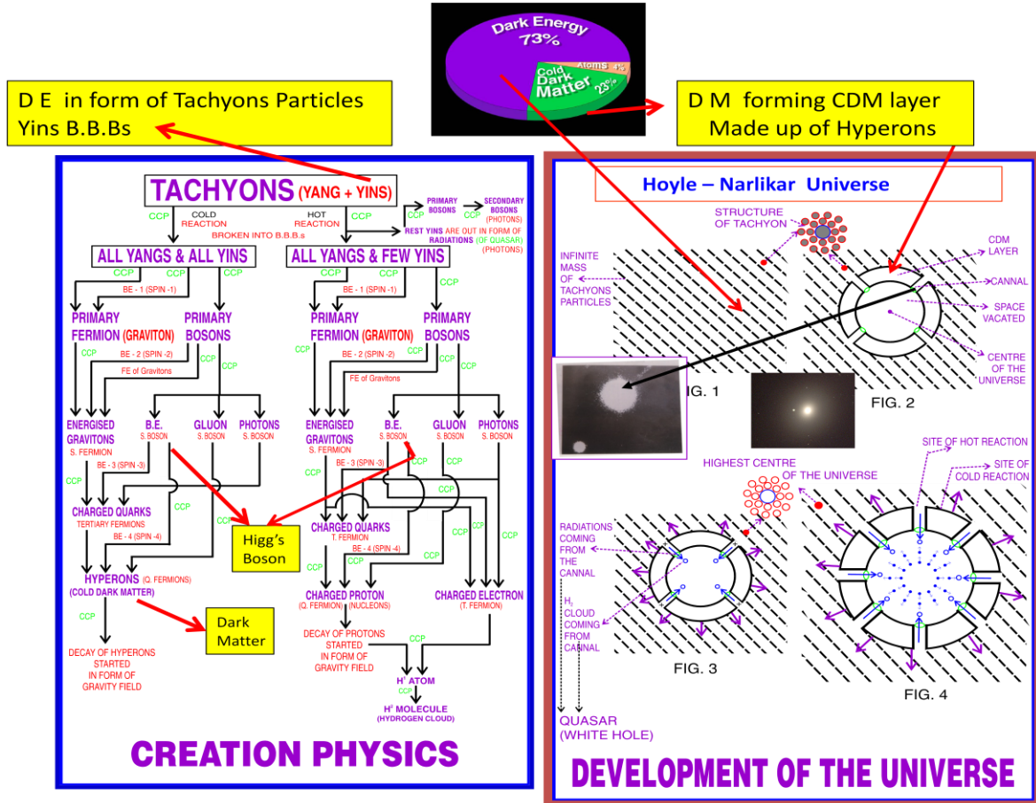
Fig 11 structural configuration of DM and DE at macro level [12]
