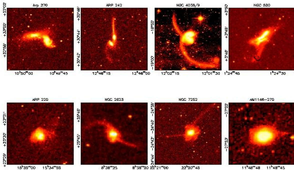
Fig 15 Two Bright Galaxies: Merging Galaxies
