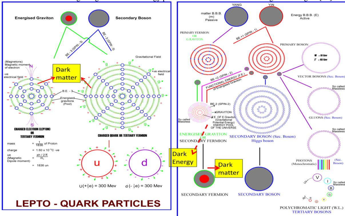
Fig. 10 Structural configuration of Leptons and Quarks as regard DM and structural configuration of DM and DE at micro level
