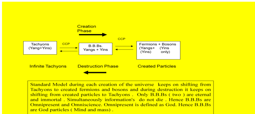
Fig .3.1 one creation and destruction cycle [7]
